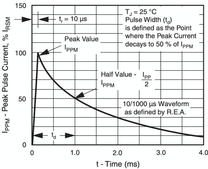
Fig.3 - Pulse Waveform
